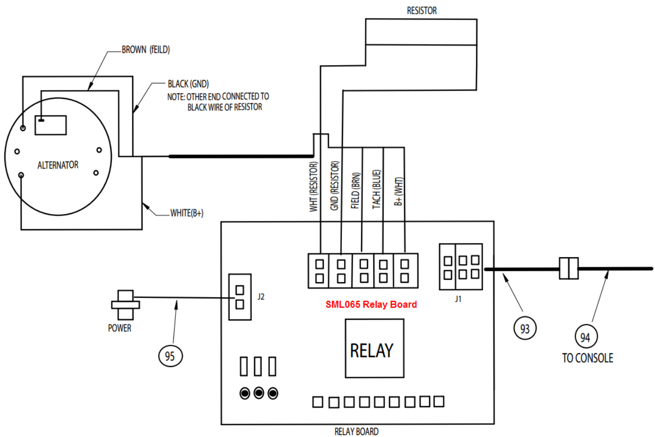
StepMill Alternator (Prestolite yellow label) Wiring Schematic
